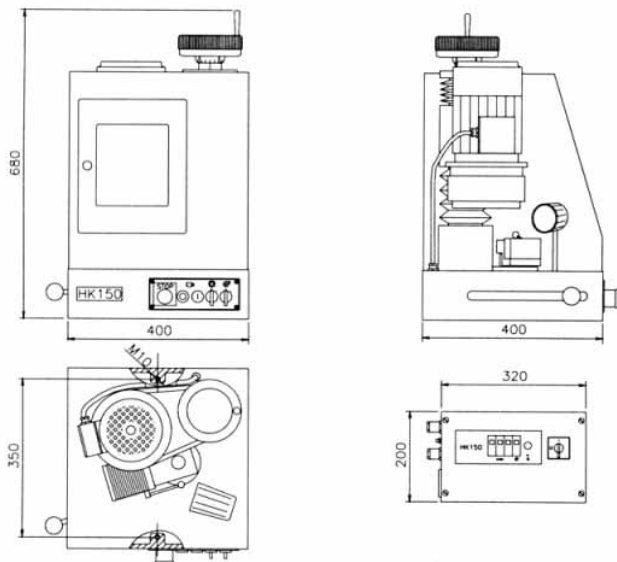
Technical drawing of HK150
